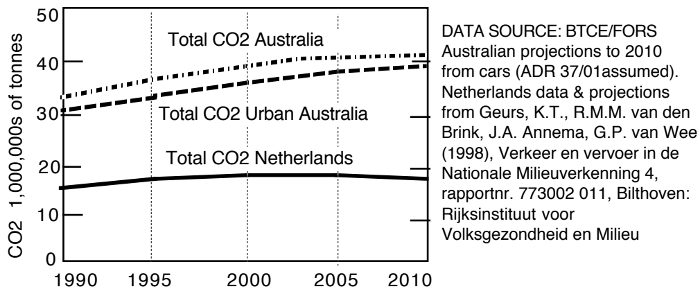
Fig 7. CO2 emissions: passenger cars: Australia and The Netherlands
